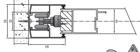
SOFFIT FIXED 100TA TRACK, 100PA PELNET AND 100TF HANGER WITH ALUMINIUM DOOR
