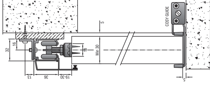
SECTION THROUGH DOOR SECTION SCALE: 1:3
