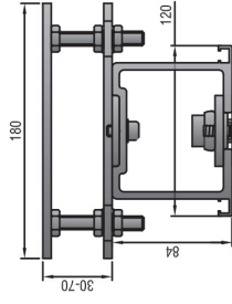
SECTION THROUGH DOOR SHOWING SOFET FIX 600TA TRACK WITH TOP SUSPENSION BRACKET AND 600P PIVOT
