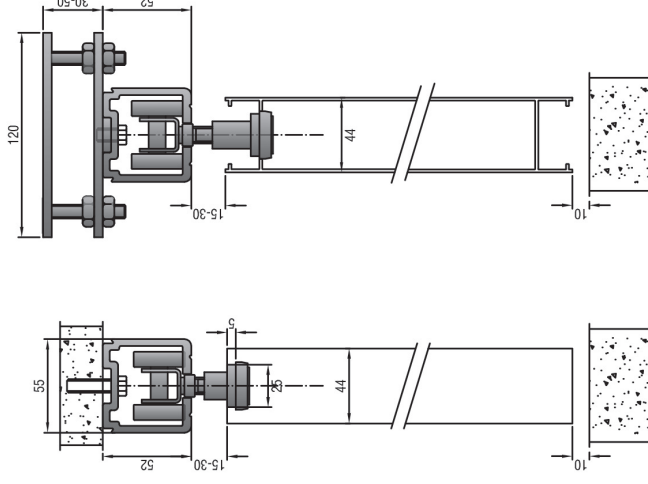
SOFFIT FIX 400TA TRACK WITH 400TP/A HANGER ON ALUMINIUM DOOR
