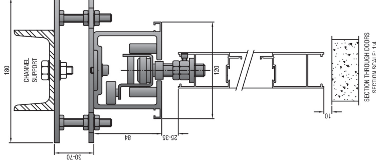
SOFFT FIX 600TA TRACK WITH TOP SUSPENSION BRACKET AND 600TF HANGER WITH ALUMINIUM DOOR
