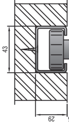
SECTION THROUGH DOOR SHOWING 19A CHANNEL WITH 805MOD GUIDE AND 815B BRASS TRACK WITH 992 BOTTOM ROLLER
