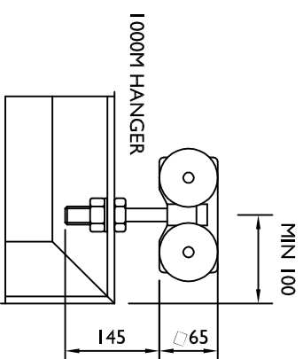
ELEVATION OF HANGER FIXING
