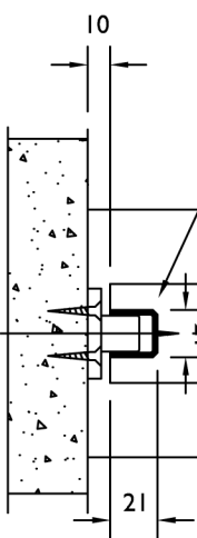
19A CHANNEL WITH 40/19N GUIDE
