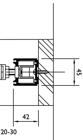
TRACK SOFFIT FIXED IN A BRICK RECESS WITH TIMBER DOOR AND 200TF TOP FIXING HANGER
