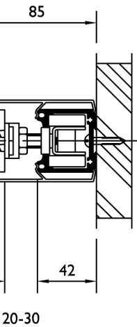
TRACK SOFFIT FIXED WITH DOUBLE CLIP-ON REBATE AND 200TF HANGER
