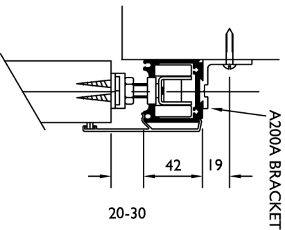
19A CHANNEL WITH 40/19N GUIDE
