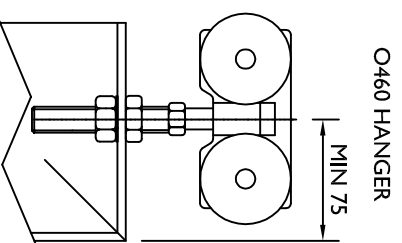
ELEVATION OF HANGER AND DOOR. USE 2 HANGERS AND 2 GUIDES PER DOOR
