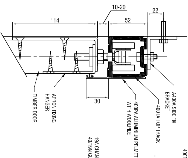
SECTION THROUGH DOOR
