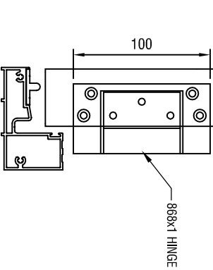
SECTION THROUGH DOOR AT HINGE
