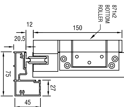
SECTION THROUGH DOOR AT ROLLER AND GUIDE
