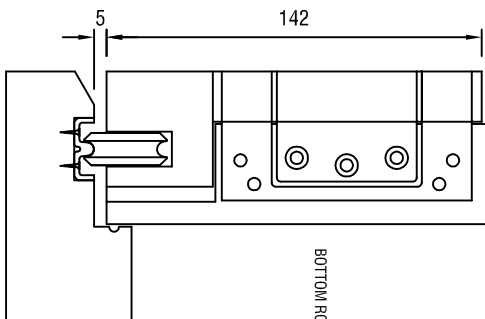
SECTION THROUGH DOOR AT ROLLER AND GUIDE
